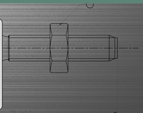
Ref.: 2005 AXIAL (CAJA RM. 17 X 1 / VASTAGO RM. 14 X 1.50) LARGO = 247 MM.
